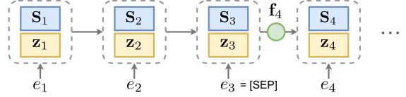
Figure 2: Our sentential gating mechanism. e_1 and e_4 are at the beginnings of two sentences.
