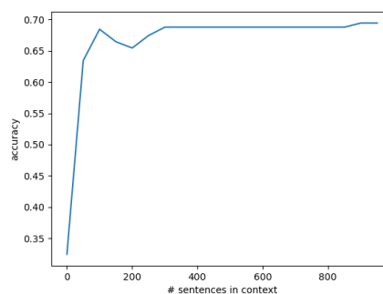
Figure 4: The accuracy on PPDB-filtered as a function of the number of contexts used by McPhraSy to represent phrases (at inference time).
