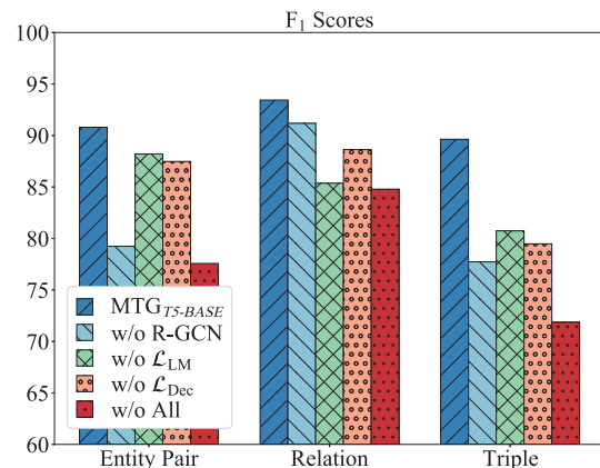
Figure 4: An ablation study on a manually selected subset with triples that require relational reasoning.
