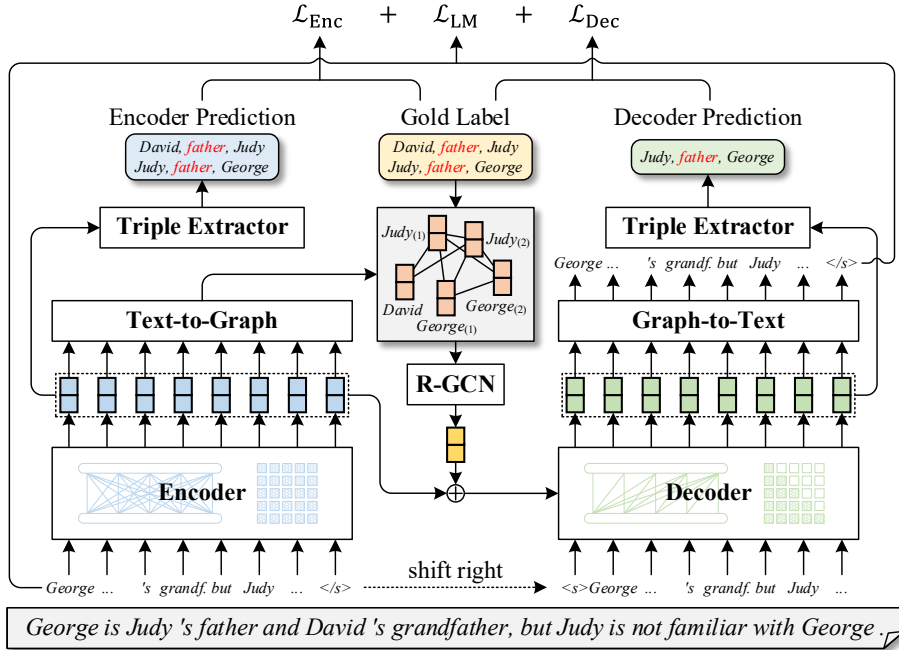
Figure 2: The overall framework of our approach. When recovering the sentence, we use the left-to-right Language Model (LM) objective, which is controlled by the lower triangular attention mask of the Transformer decoder.
