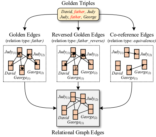
Figure 3: An example of the relational graph edges.
