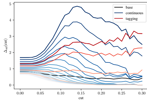
Figure 3: How we can vary monotonicity \text{EN} \Rightarrow \text{DE} for different interventions. The model using tagging is \text{Tag}(L, M, P_d) while the continuous model is \text{Add}(L, M_{0.1}, P_c) . Darker shades of the same color represent larger values of the intervention \delta .
