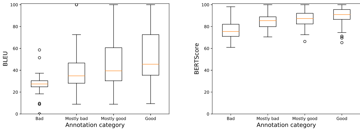
Figure 1: Box plots of BLEU (left) and BERTScore (right) for English showing the distribution of sentence-level scores for each annotation category. The annotation categories are introduced in Section 4.1.
