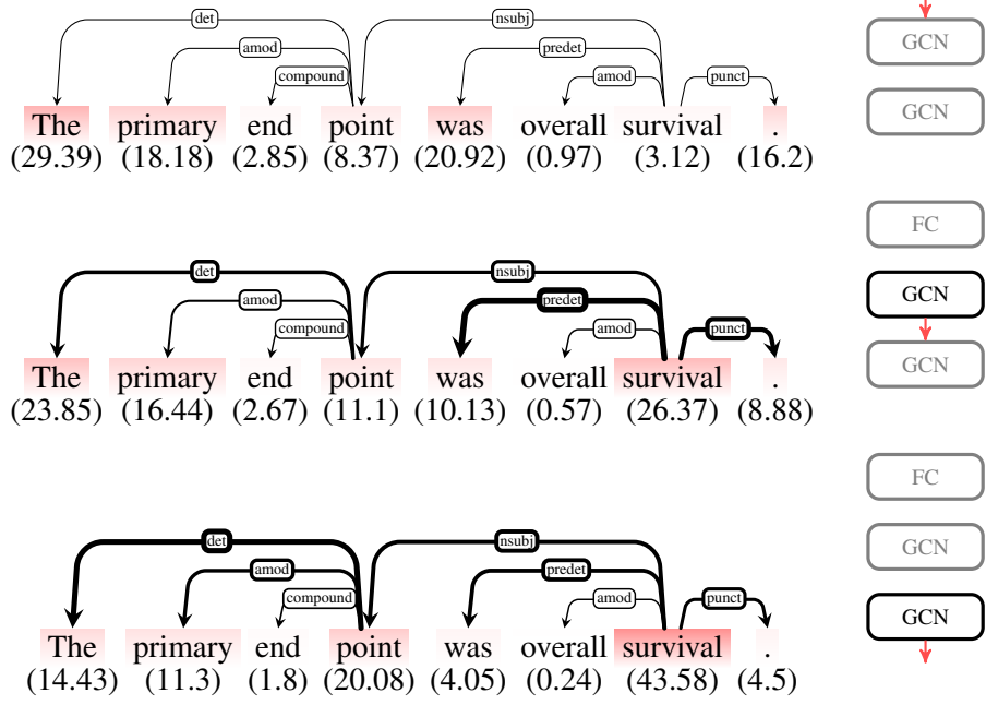
Figure 3: Predicted label: METHOD, true label: METHOD.
