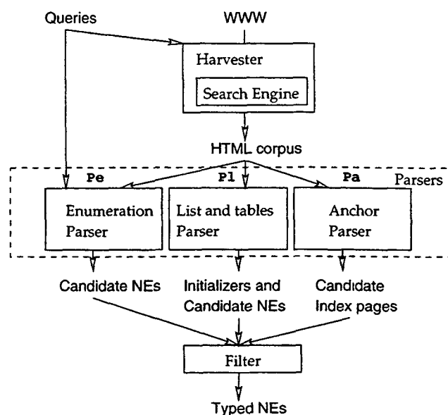
Figure 1: Architecture
