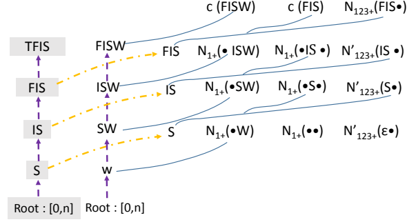
Figure 5: Example MKN probability computation for a 4-gram LM applied to “ The Force is strong with ” (each word abbreviated to its first character), showing in the two left columns the suffix matches required for the 4-gram FISW and elements which can be reused from previous 4-gram computation (gray shading), TFIS. Elements on the right denote the count and occurrence statistics derived from the suffix matches, as linked by blue lines.
