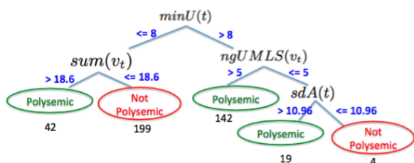
Figure 3: Decision Tree.
