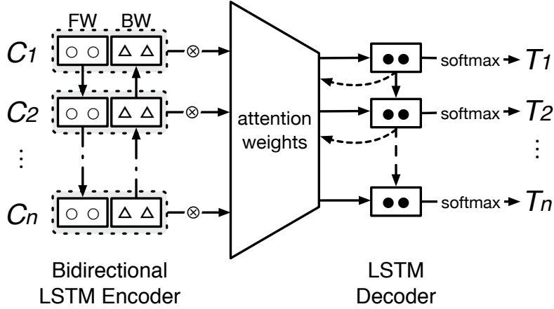
Figure 1: Overview of the encoder-decoder model with attention mechanism. Character embeddings C_1 to C_n of the input sentence is sequentially fed into the bidirectional LSTM, and the concatenated output is multiplied by attention weights and sent to the decoder for predicting the tag sequence T_1 to T_n . For simplicity, multiple layers of encoder and decoder as well as dropout layers between them are omitted.
