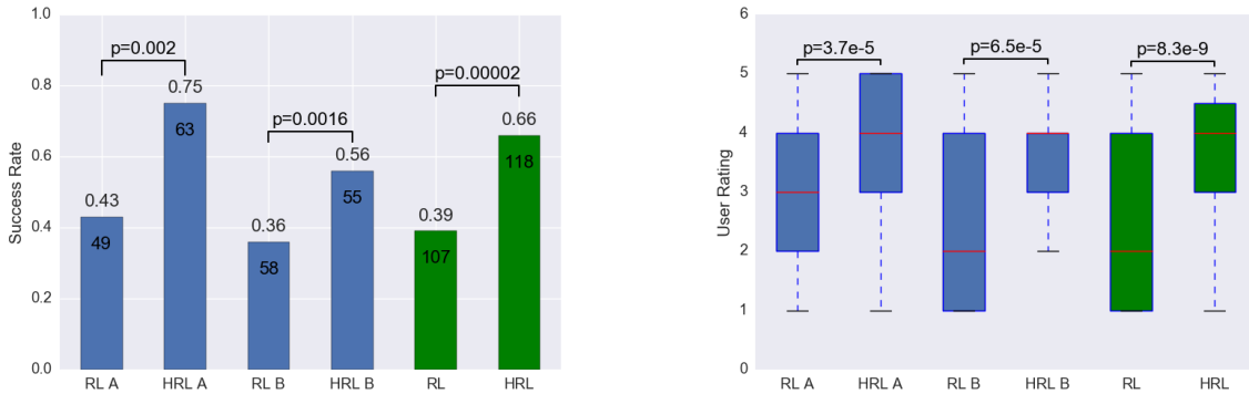
Figure 5: Performance of HRL agent versus RL agent tested with real users: success rate, number of tested dialogues and p-values are indicated on each bar; the rightmost green ones are for total (difference in mean is significant with p < 0.01 ).
