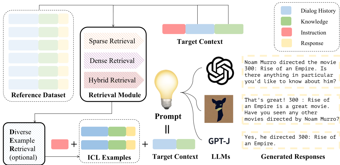
Figure 2: An overview of IKA framework.
