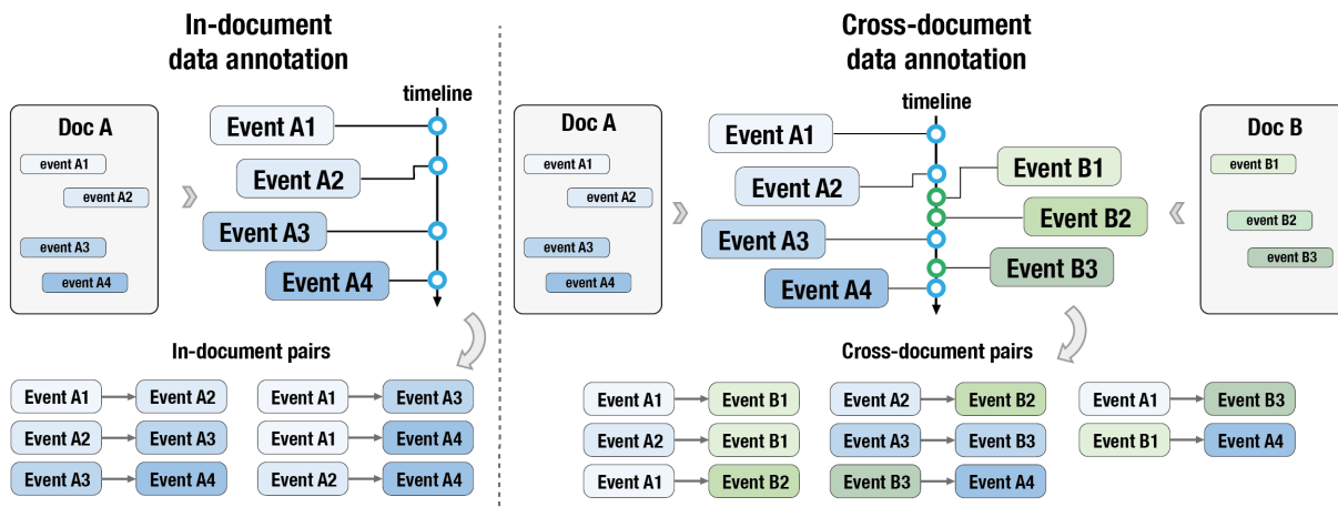
Figure 4: Dataset construction pipeline. Once events are extracted from the documents (Section 3), we order them on time and formulate story timelines. Conditioned on the temporal ordering, we create all combinations of events in the document and pass the in-document pairs to annotators. We perform a similar process for the event pairs extracted from different documents (cross-doc), including an extra step of merging document timelines into one before taking the pair combinations.
