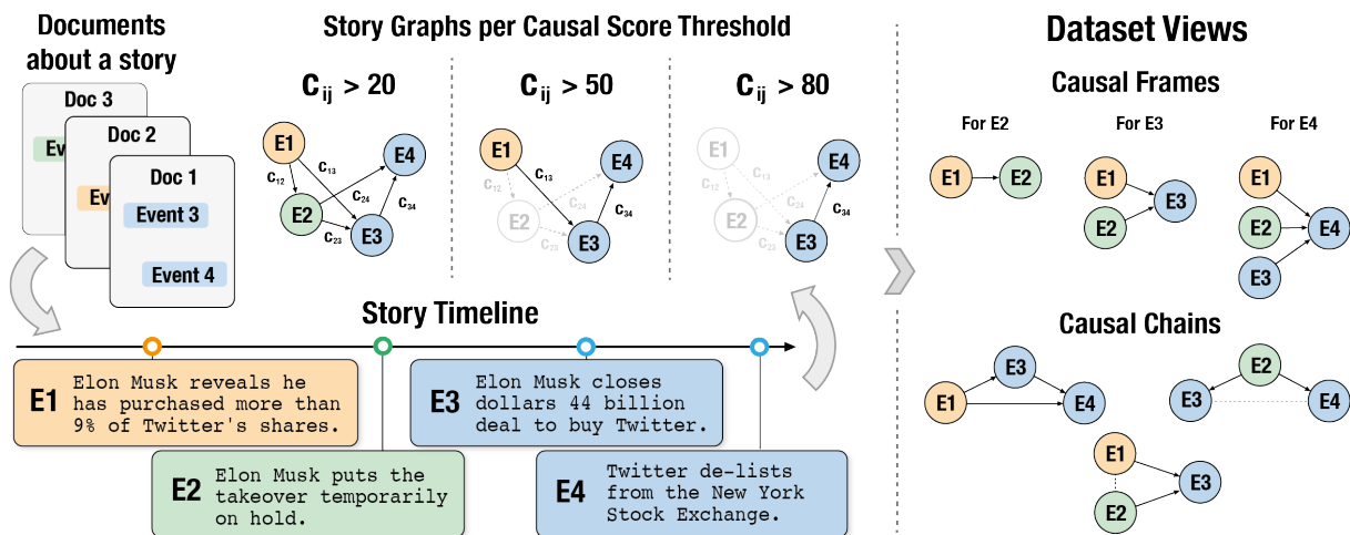
Figure 3: CRAB data pipeline overview: We collect documents covering newsworthy stories, create a timeline with the main events extracted from the documents for each story, and crowdsource human annotations on the causal judgments between the events ( score 0 to 100 ). Based on these scores, we generate a causal graph for each story that can be filtered on different causal score thresholds. CRAB can also be viewed from the perspective of causal frames and causal chains as presented in Section 2. Same-color events originate from the same document.
