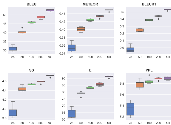
Figure 2: Boxplots for selected metrics from Table 2 w.r.t. the number of examples (displayed on the x-axis, full = 1522), taking into account variance from individual random seeds (cf. Table 6).
