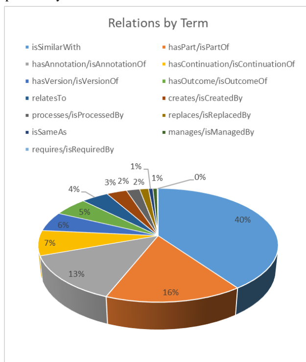
Figure 4: Chart showing relations by term, sorted most to least frequently occurring. Data is from 2000-2020. Note isPartWith is not represented in this chart since it is automatically generated.
