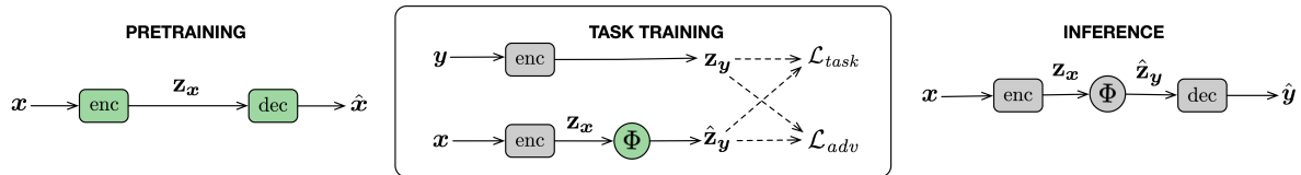
Figure 2: High-level view of the supervised variant of our framework Emb2Emb . Left : we pretrain an autoencoder on (unannotated) text, which transforms an input sentence x into an embedding z_x and uses it to predict a reconstruction \hat{x} of the input sentence. Center : using the (frozen, hence depicted in gray) autoencoder, we learn a mapping \Phi (trained, hence depicted in green) from the autoencoder’s embedding of an input z_x to the embedding z_y of the output sentence y . The training objective consists of two losses: \mathcal{L}_{task} enforces the predicted output embedding to be close to the true output embedding, and \mathcal{L}_{adv} is an adversarial loss term that enforces the output embedding to be on the manifold of the autoencoder. Right : at inference time, \Phi is composed between the autoencoder’s encoder and decoder to transform input sentence x to output sentence \hat{y} . Not shown: the unsupervised variant where only x (not y ) sequences are available in task training (Section 9).
