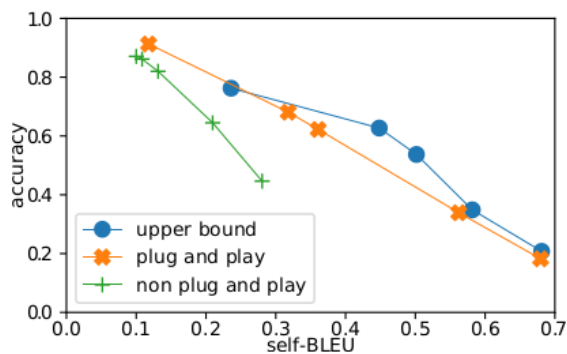
Figure 6: Sentiment transfer results for different model scenarios. Up and right is better.
