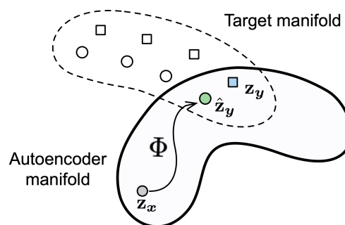
Figure 1: The manifold of a text autoencoder is the low-dimensional region of the high-dimensional embedding space where texts are actually embedded. The example shows the mapping of a source sequence x with embedding z_x to z_y , which is the embedding of target sequence y such that it reflects the target manifold.
