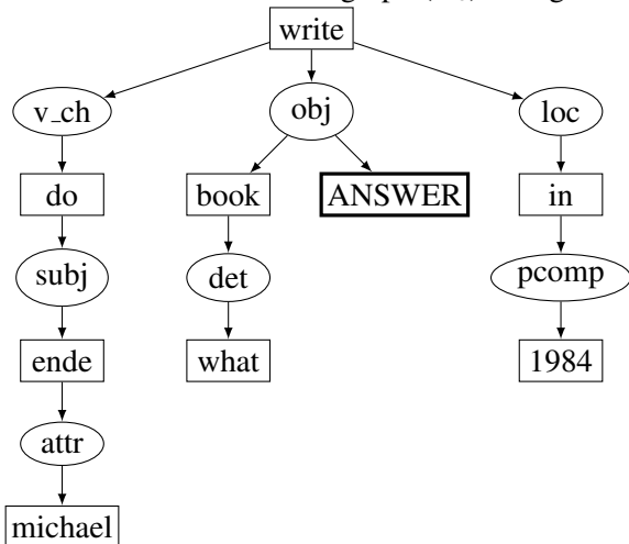
Figure 3: Example of a QA rule. R_p is in solid lines, R_e is in dashed lines, and R_a is in thick lines.
