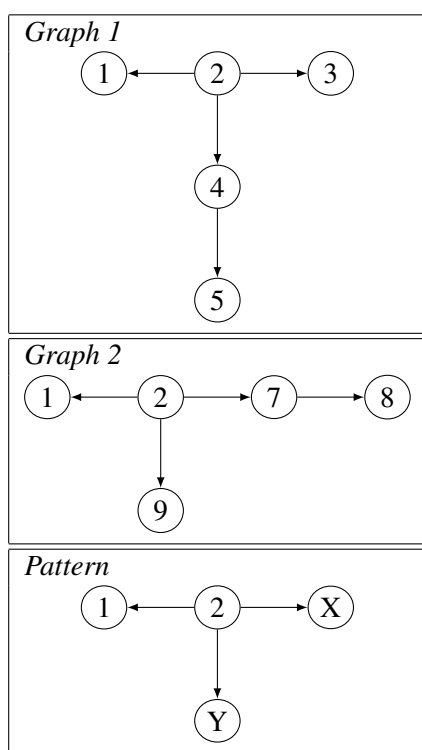
Figure 1: Two graphs and a pattern (variables in uppercase)
