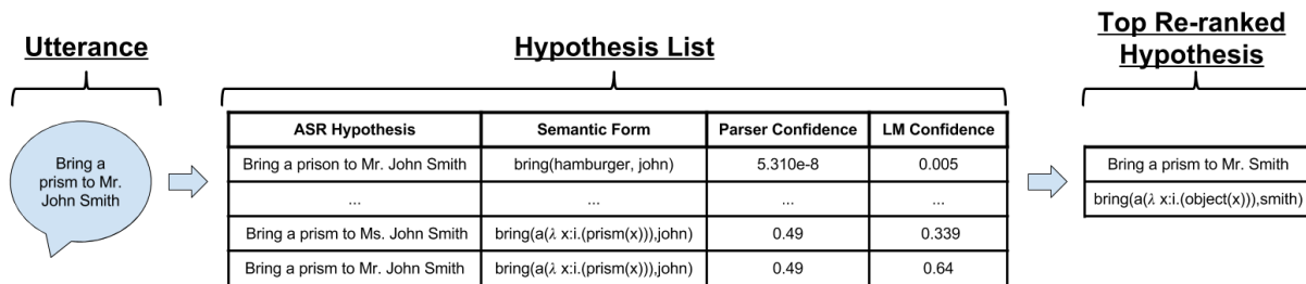
Figure 1: Our proposed methodology. The black-box ASR outputs an ordered list of its top hypotheses. Each hypothesis is given confidence scores by an in-domain semantic parser and language model, which are then used to re-rank the list. In this example, the parser has learned that “Mr.” and “Ms.” are functionally equivalent, while the language model has learned that “Mr.” co-occurs with “John” more than “Ms.” does. Together, they guide us to select the correct transcription.
