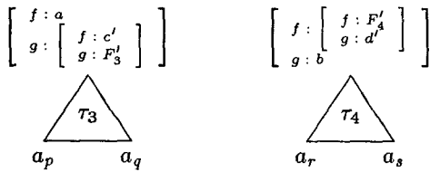
Figure 8: Compatible subderivations
