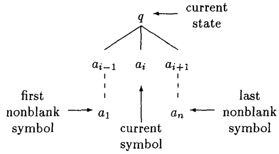
Figure 3: Encoding a Turing Machine
