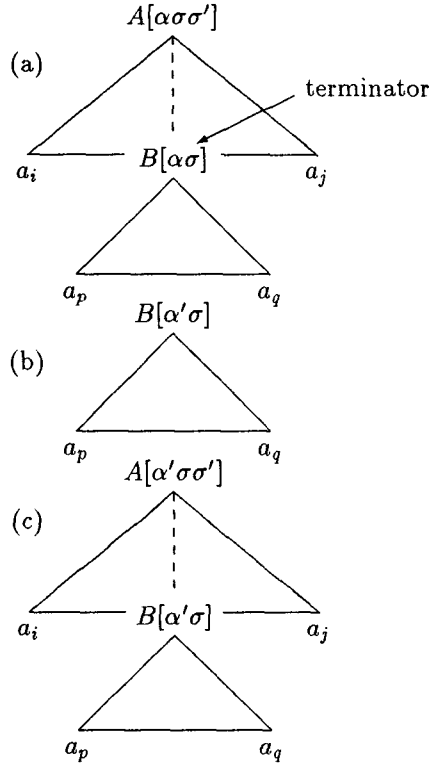
Figure 6: “Context-Freeness” in LIG derivations
