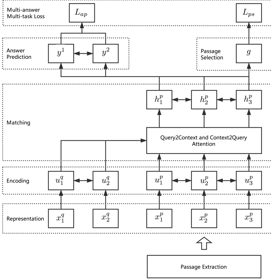
Figure 2: Model Architecture
