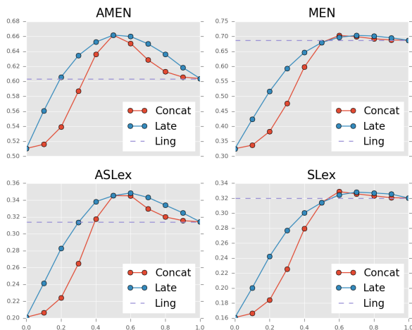
Figure 1: Performance of middle and late multi-modal fusion models compared to linguistic representations on the four datasets when varying the \alpha mixing parameter on the x-axis.
