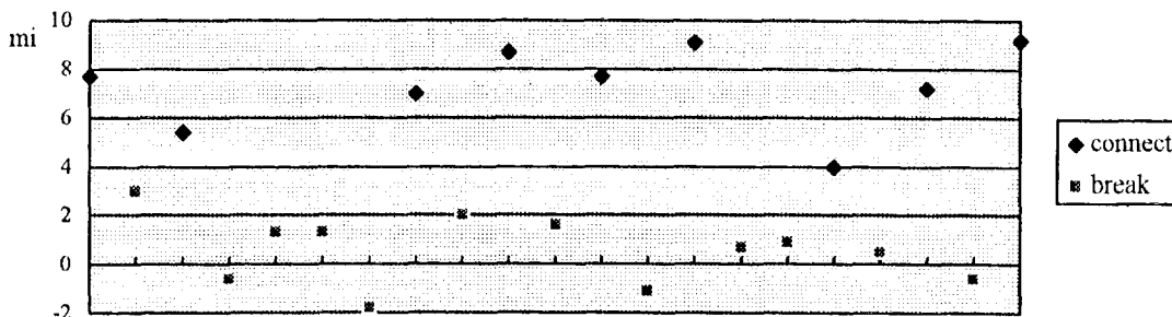
Fig.1 The distribution of mi(sentence 1) Character pairs in sentence
