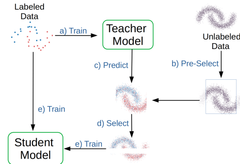
Figure 1: Pseudo-Labeling Framework. After teacher model training (a), it is used to predict pseudo-labels (c) for pre-selected unlabeled data points (b). After the selection of reliable pseudo-labels (d), a student model is trained with labeled and pseudo-labeled data (e).
