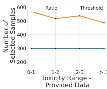
(d) While the number of selected samples slightly drops with increasing hate ratio for the threshold-based approach, the number remains constant for the ratio-based approach.
