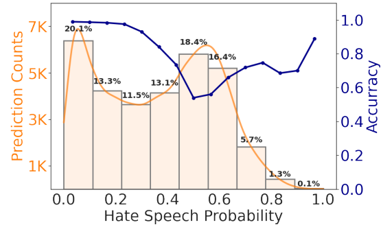
Figure 2: Histogram and accuracy values of our baseline model with respect to hate speech probabilities, which have been computed over all unlabeled data samples of the seed dataset. The model tends to make more predictions in favor of the normal class. Moreover, these predictions have a higher degree of accuracy than the hate speech class.
