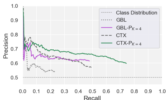
Figure 6: Experiment 1: LM smoothing on the ANT dataset. Comparison of P-smoothing GBL and CTX with optimal K=4 .
