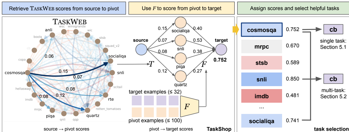
Figure 2: Overview of single and multi-task selection using TASKSHOP and TASKWEB. Section 3 describes the pairwise task transfer involved in TASKWEB as well as its analysis. Section 4 details TASKSHOP and describes task selection in single task and multi-task setups. Section 5 presents our experiments as well as additional analyses.
