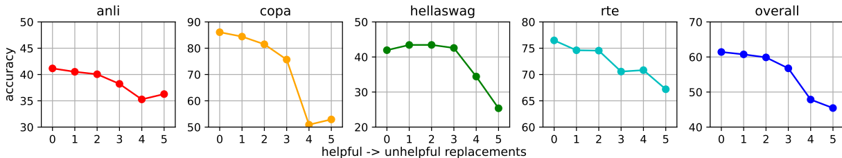
Figure 4: Variations in the zero-shot target performance as the top-5 source tasks for each target are incrementally replaced by the bottom-5 source tasks according to TASKWEB while maintaining the size of the training set.
