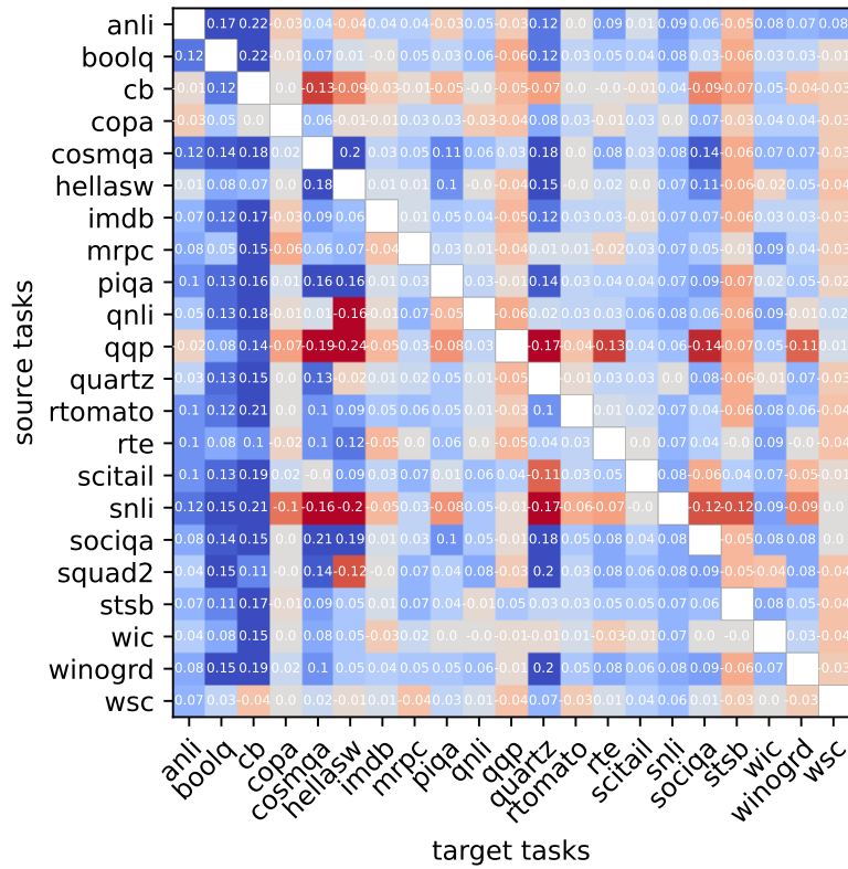
Figure 6: Visualization of pairwise transfer between 22 different NLP tasks for T5-large (Raffel et al., 2020) finetune. We display the actual transfer scores, with positive transfers in blue and negative transfers in red.
