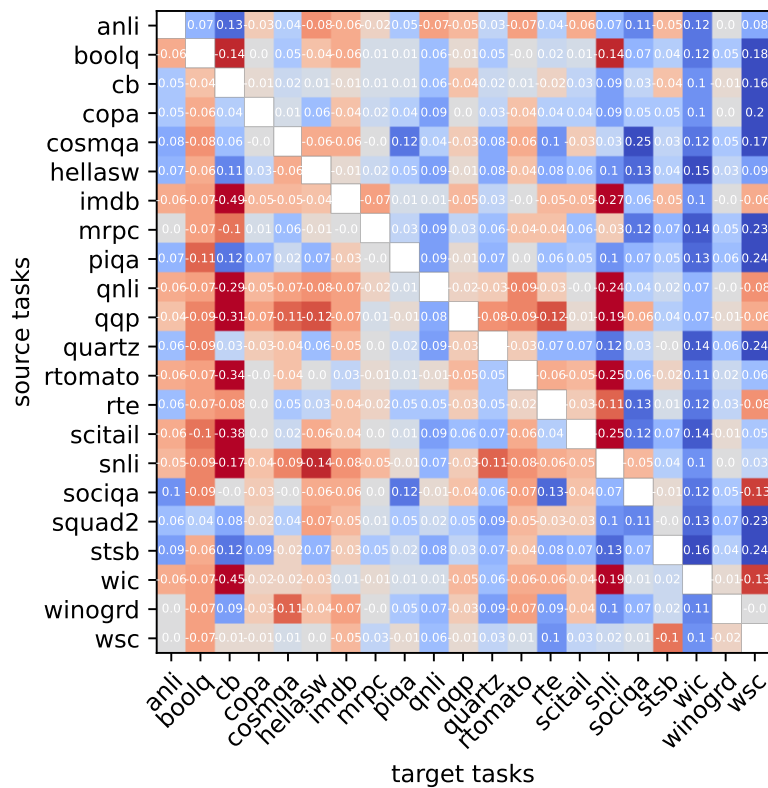
Figure 9: Visualization of pairwise transfer between 22 different NLP tasks for GPT-2 medium (Radford et al., 2019) finetune. We display the actual transfer scores, with positive transfers in blue and negative transfers in red.
