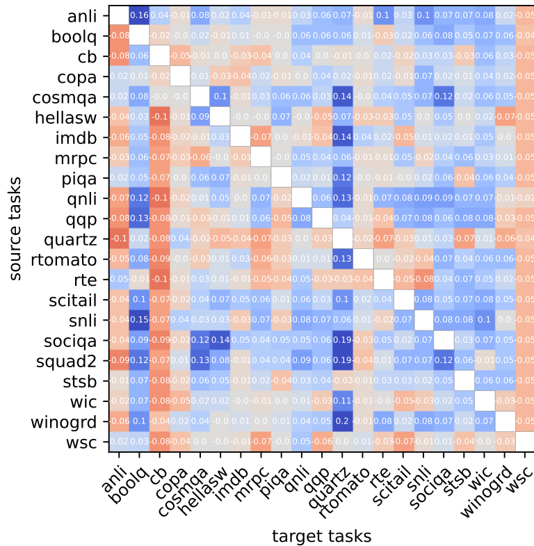
Figure 7: Visualization of pairwise transfer between 22 different NLP tasks for T5-base finetune. We display the actual transfer scores, with positive transfers in blue and negative transfers in red.
