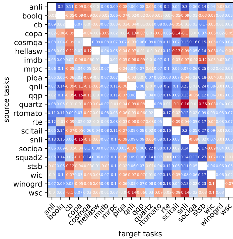
Figure 11: Visualization of pairwise transfer between 22 different NLP tasks for T5-base BitFit (Zaken et al., 2022). We display the actual transfer scores, with positive transfers in blue and negative transfers in red.
