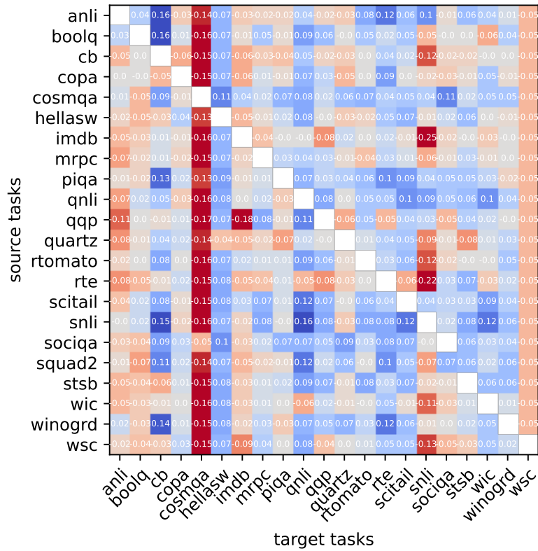
Figure 10: Visualization of pairwise transfer between 22 different NLP tasks for T5-base adapters (Houlsby et al., 2019). We display the actual transfer scores, with positive transfers in blue and negative transfers in red.
