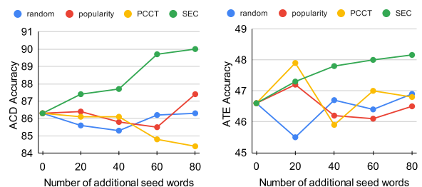
Figure 4: ACD and ATE performances with different seed word addition strategies. Our baselines: random adds seed words randomly from the vocabulary, mapped to their aspects by Eq.2, while popularity selects the most frequently occurring important words (noun/adjective) of each aspect based on a small labeled dataset (dev set). PCCT is a set of additional seed words proposed by (Li et al., 2022), extracted from the vocabulary of a pre-trained model.
