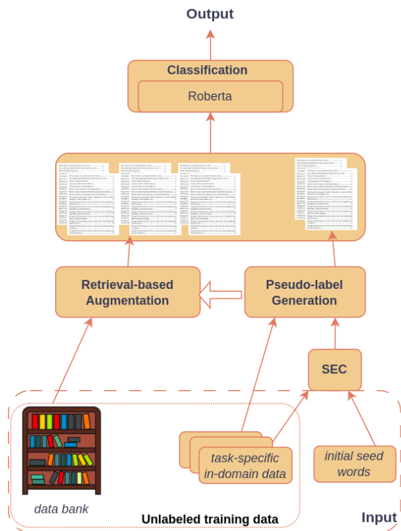
Figure 1: Overview of our proposed Self-enhancement Multitask (ASeM) framework.
