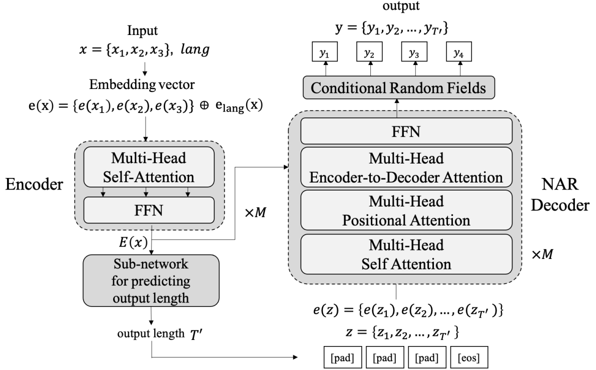
Figure 1: The overview of proposed model
