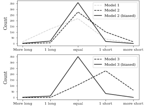
Figure 4: Results with predicted output length (biased or not)
