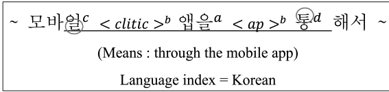
Figure 2: The example of composition of features for each token in a sentence
