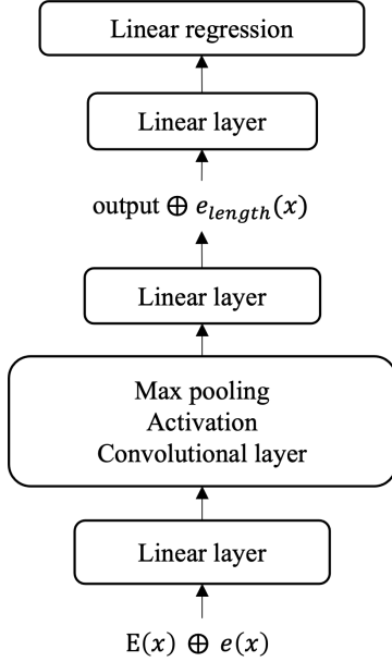
Figure 3: The sub-network for predicting and using output length
