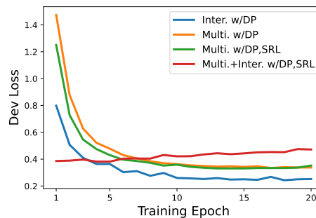
Figure 6: The loss curve on development set of AMR 2.0 for different training paradigms.
