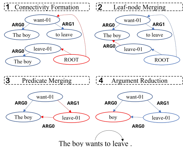
Figure 4: Illustration of Dependency Guided Restoration. In step 2, leaf-nodes “The boy” are merged. In step 3, none-leaf node “leave-01” is merged with leaf-node “to leave” since “leave-01” appears in word span “to leave” and word “leave” depends on word “want”.
