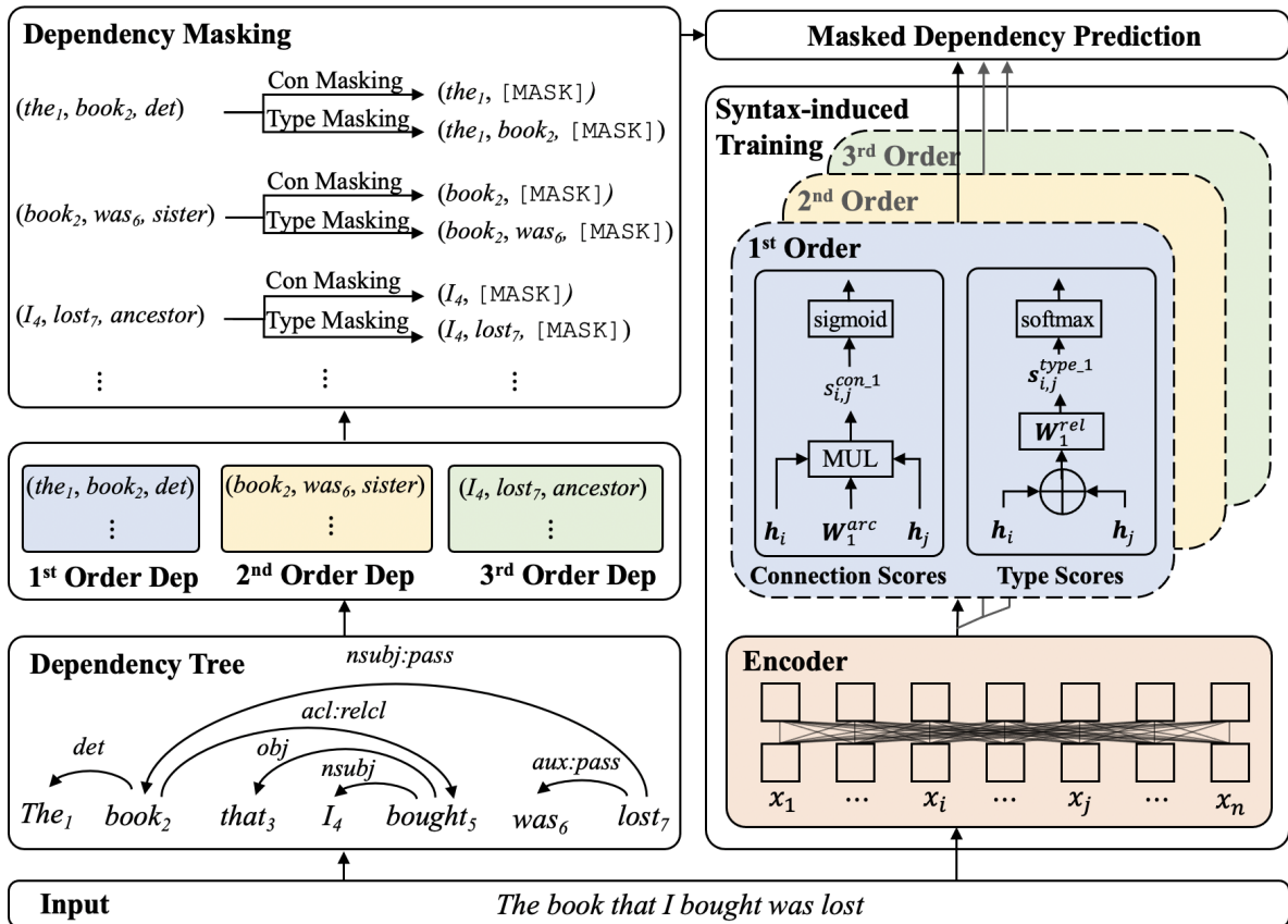
Figure 1: An overview of our approach to train a syntax-induced encoder (highlighted in the red box). The left part shows the process to extract and mask dependencies (connection and type masking, respectively) in first, second, and third orders, where the word subscript denotes its sentential index. The right part illustrates the process to compute the scores of dependency connections and types in different orders to recover the ones that being masked.
