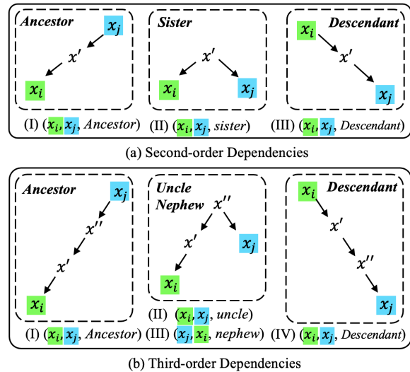
Figure 2: An illustration of the three second-order (a) and four third-order (b) dependency types between x_j and x_i , based on their positions in the parse tree.
