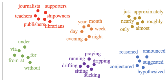
Figure 5: Visualizations of the learned representations through the syntax-induced encoder for some example words. The distance between any two words illustrates their similarity in terms of syntax and semantics. Words are presented in clusters and those in the same cluster are represented in the identical color.
