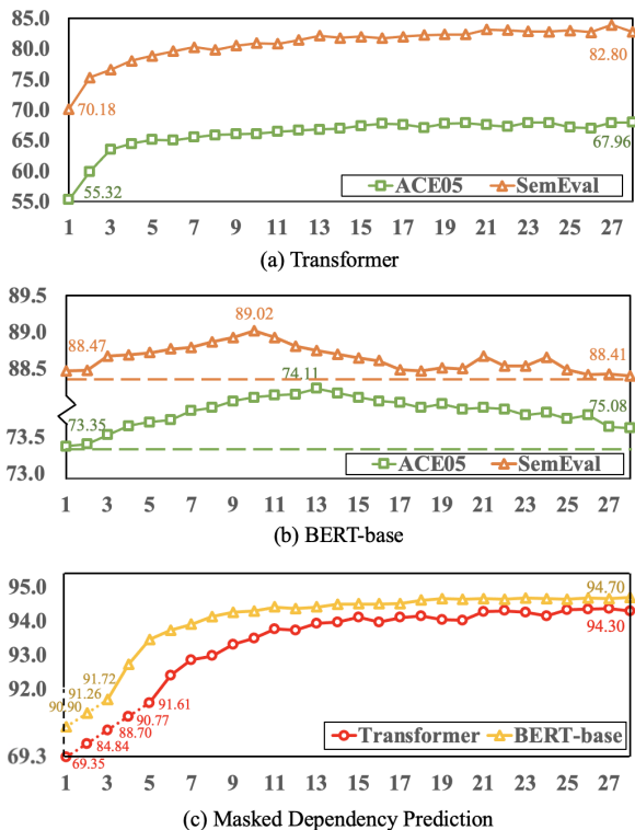
Figure 4: Curves of fine-tuning different base encoders (Transformer (a) and BERT-base (b)) on ACE05 and SemEval with respect to the number of training steps (in 100K). For reference, (c) shows the dependency parsing performance (LAS) of the learned encoders (Transformer and BERT-base) on the test set of English Penn Treebank (PTB) against its pre-training steps, where higher scores suggest that more intensive introduction of dependency information.
