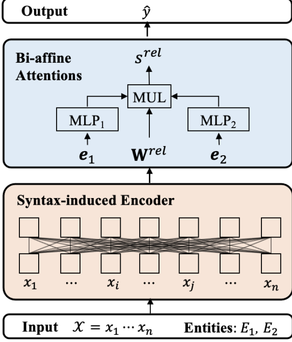
Figure 3: The architecture of our model for RE with the syntax-induced encoder (highlighted in red color) pre-trained on auto-parsed data through DMP.
