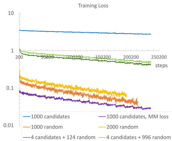
Figure 5: Evolution of the loss on the training set, as training of BM25→CODER(RepBERT) progresses. Different curves correspond to a different type and number of documents used as negatives during training. While training loss is decreasing in all cases, only using numerous retrieved candidates as negatives, combined with a list-wise KL-divergence loss, results in a significant improvement of performance over the base method (see Figure 2) on the validation and test sets.
