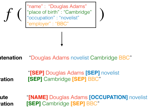
Figure 1: Shown here are three ways of representing an entity with arbitrary attribute-values (Section 4.1). Concatenation simply concatenates all values, [SEP]-separation separates values using [SEP] tokens, and attribute separation introduces special tokens based on frequently occurring attributes (which in this example are “name” and “occupation”).
