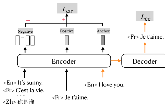
Figure 1: The proposed mRASP2. It takes a pair of parallel sentences (or augmented pseudo-pair) and computes normal cross entropy loss with a multi-lingual encoder-decoder. In addition, it computes contrastive loss on the representations of the aligned pair (positive example) and randomly selected non-aligned pair (negative example).
