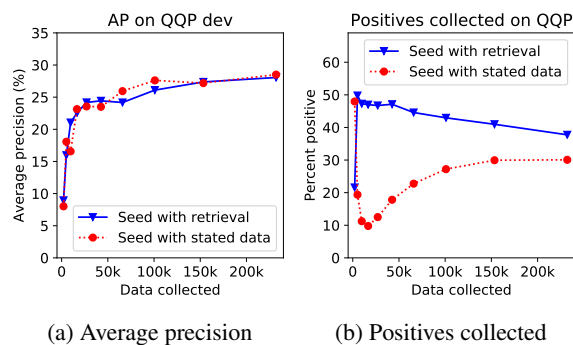
Figure 3: Uncertainty sampling on QQP using different seed sets. (a) Seeding with stated data (one run) does similarly to seeding with retrieval (mean over three runs). (b) Seeding with stated data makes the model poorly calibrated—points it is uncertain about are initially very unlikely to be positive. However, over time the model corrects this behavior.
