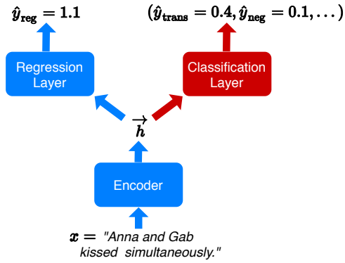
Figure 1: Illustration of the methodological framework for symmetry inference. The blue modules represent regression learning pipeline for each single model, and Stage 2 of the hybrid model. The red module denotes Stage 1 of the hybrid model in transfer learning.
