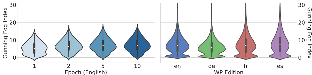
Figure 4: Kernel density estimated Gunning Fog distributions and box plots over extracted en ( en-de ) sentences at different points in training (left) and over the monolingual Wikipedias (right).
