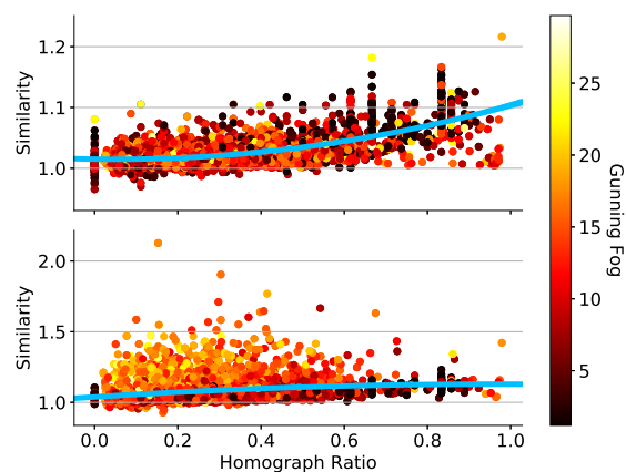
Figure 5: Margin-based similarity, homograph ratio and Gunning Fog index for the first 10 k extracted sentences in the first (top) and last (bottom) epoch of en-fr training. The solid blue line shows a second order polynomial regression between the homograph ratio and similarity.
