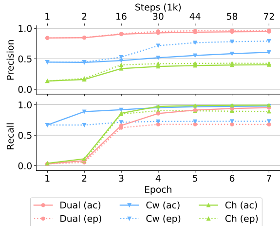
Figure 1: Accumulated (ac) and epoch-wise (ep) precision and recall on the en-fr EP-based synthetic comparable data.
