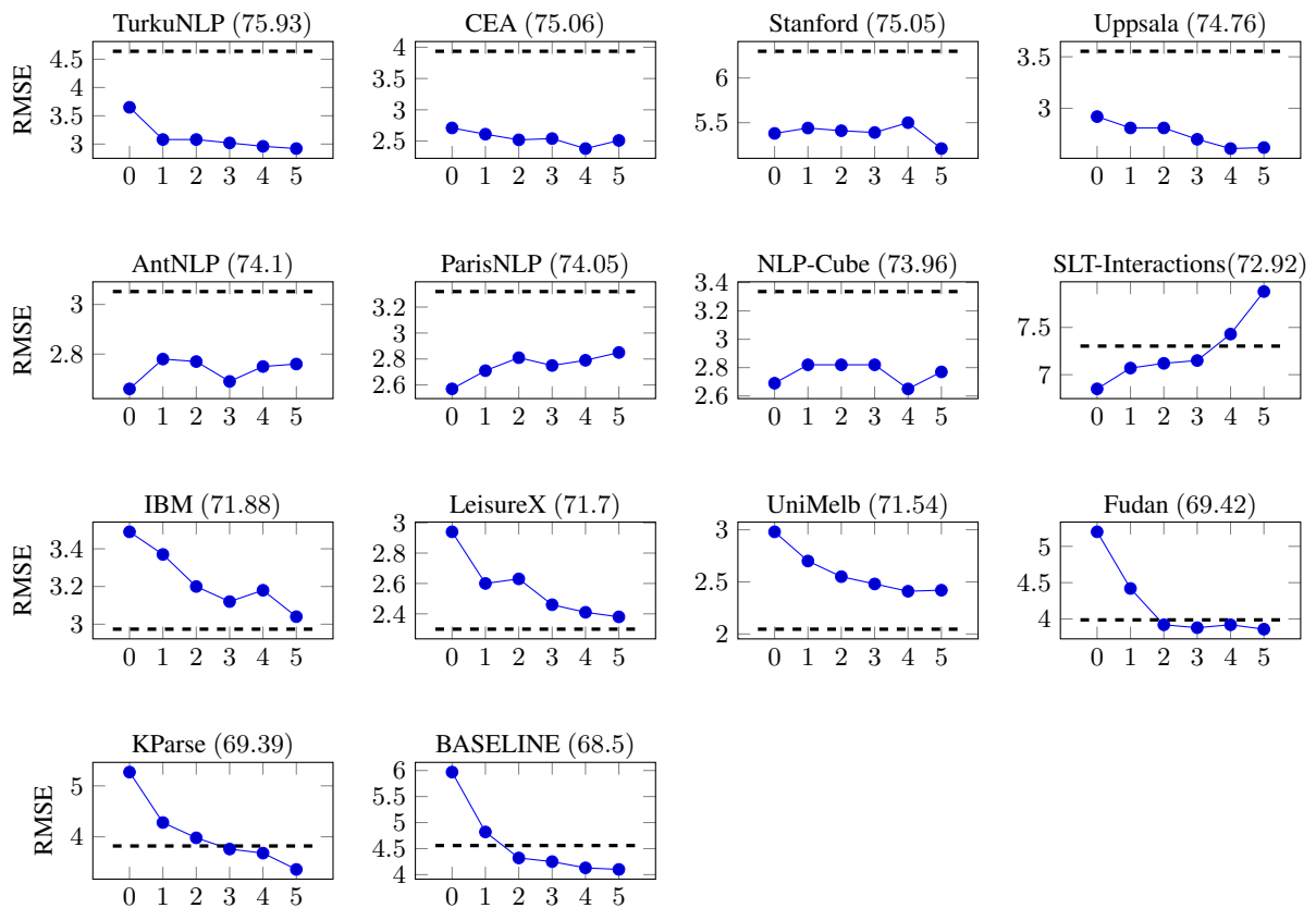
Figure 7: RMSE scores of UD task from dataset-wise mean value predictor (the dashed black line in each graph) and predictors trained with experimental records of other models and 0–5 records from a new model (as indicated by the title of each graph).
