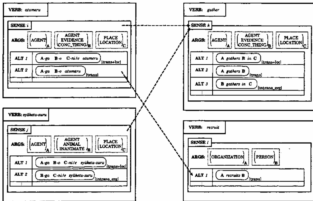
Figure 6: The separated and relinked dictionary
