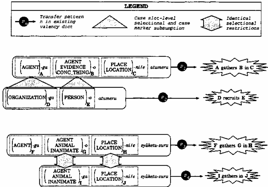
Figure 1: Japanese-English sense correspondence
