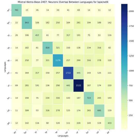
Figure 11: Mistral Nemo: Language neuron overlap between languages using LAPE in a set of languages \{en, bn, hi, ur, mr, pa, ta, te, ml, kn\} .
