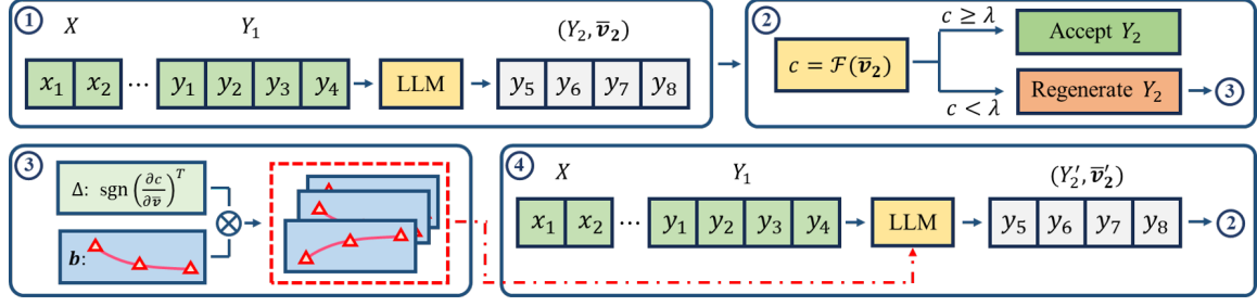
Figure 4: Illustrated example on the generation of one chunk of output in GAME. Step ① : the LLM predicts the next chunk ( Y_2 ) and calculates the chunk attention feature ( \bar{v}_2 ) without any attention editing. Step ② : the classifier ( \mathcal{F} ) predicts the hallucination score ( c ) for the generated chunk with the corresponding feature. If the score exceeds a predefined threshold, the chunk will be accepted. Otherwise, attention editing will be applied to regenerate the chunk. Step ③ : the attention edit signal for each head is computed with the prior bias and the edit direction \Delta derived from the gradient of the score. Step ④ : a new chunk is generated with the calculated attention editing signal and re-evaluated with the classifier. If no qualified chunk is accepted with number of regeneration attempts, the chunk with the highest score during the generation process will be accepted.
