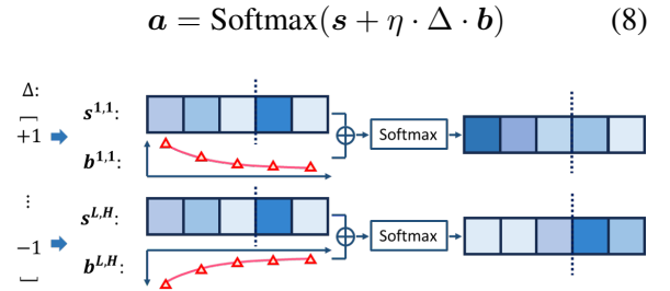
Figure 6: Illustrated example for the combination of prior attention bias and edit direction to perform attention editing.
