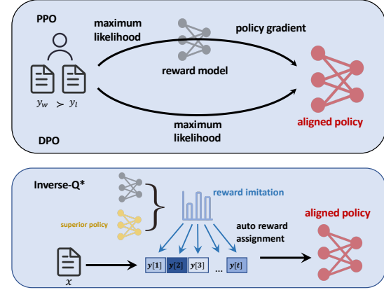
Figure 1: Existing model alignment approaches require preference data for reward modeling. However, Inverse Q* utilize reward imitation from superior strategies to achieve token-level credit assignment, making model alignment more efficient without preference data.
