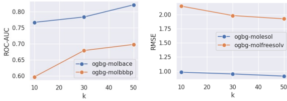
Figure 5: Ablation study of LLMCORR with a different number of contextual knowledge data ( k ) on ogbg-molbase and ogbg-molesol datasets.
