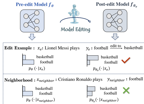
Figure 1: Existing methods can negatively impact irrelevant neighborhood examples.
