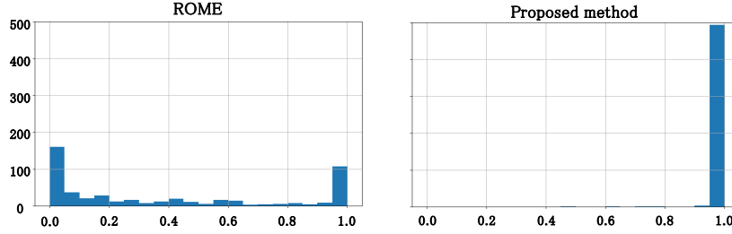
Figure 3: Histogram of p(o^*|s, r) after editing for English LLM.
