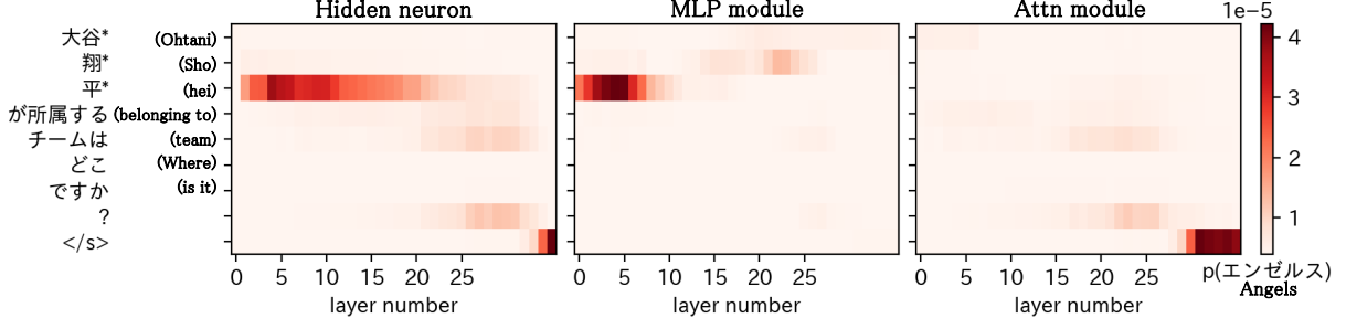
Figure 5: Indirect effect of each neuron’s activation on the probability of outputting “Angels” given the subject “Ohtani” and the relation “team” ( p(o=\text{“Angels”}|s=\text{“Ohtani”}, r=\text{“team”}) ) in each layer of the Japanese LLM (proposed method).
