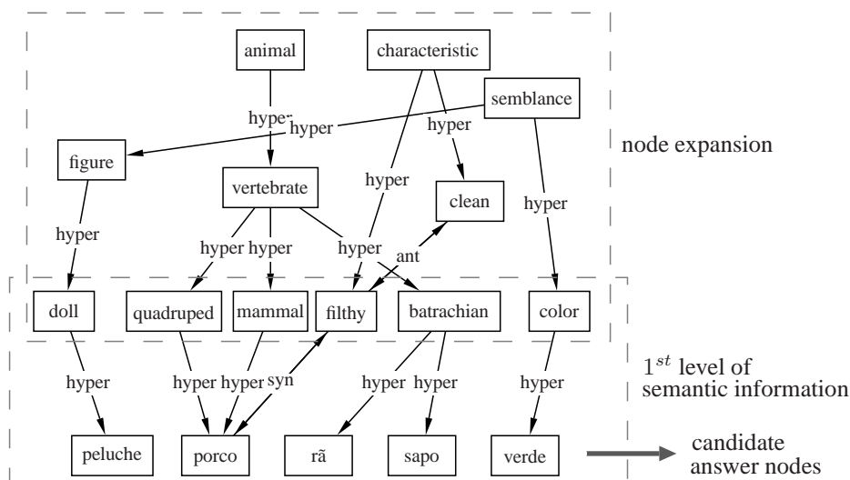
Figure 1. Candidate answers semantic network
