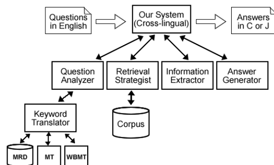
Figure2: Javelin Architecture with Cross-Lingual Extension
