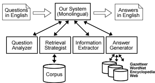
Figure1: Javelin Monolingual Architecture
