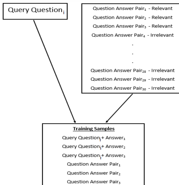
Figure 2. Generating LM training samples
