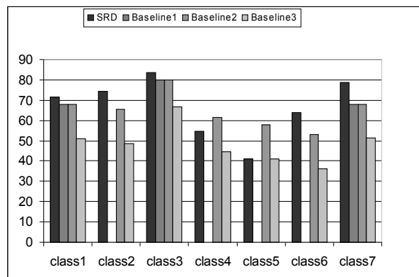
Figure1. Comparison of SRD’s F-scores for each semantic relation and the corresponding baselines.
