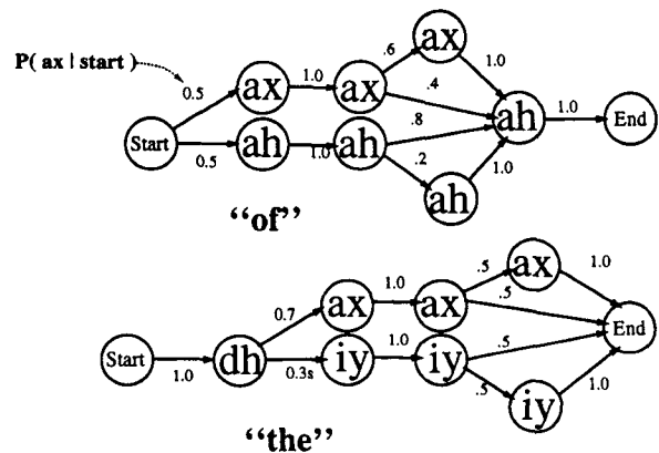
Figure 3: Pronunciation models for "of" and "the"
