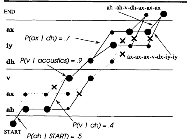
Figure 4: Computing most-likely phone paths in a Forced-Viterbi alignment of ‘of the’
