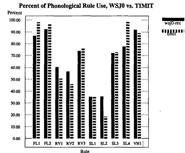
Figure 7: Automatic vs Hand-transcribed Probabilities for Phonological Rules
