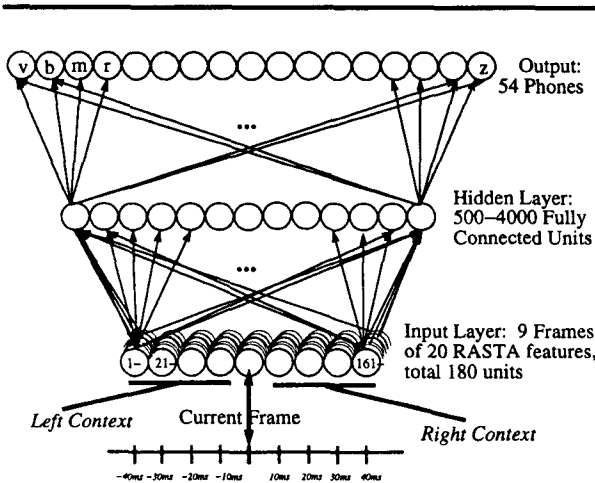
Figure 2: Phonetic Likelihood Estimator
