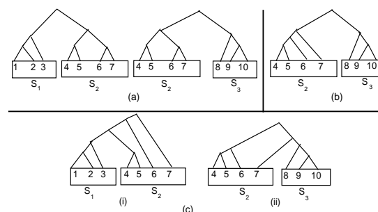
Figure 8: Extracting sub-trees for S_2 .
