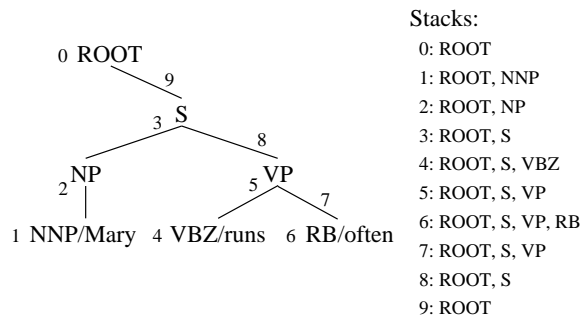
Figure 1: The decomposition of a parse tree into derivation decisions (left) and the stack after each decision (right). The derivation is shift(NNP/Mary) , project(NP) , project(S) , shift(VBZ/runs) , project(VP) , shift(RB/often) , attach , attach , attach .
